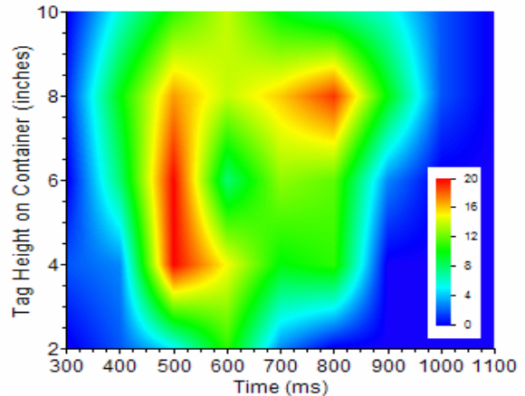
Figure 11: Conveyor performance at different heights
