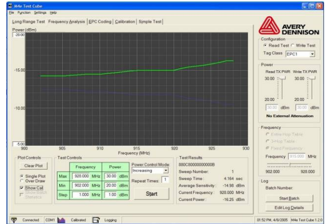
Figure 5: Test cube link margin plot
