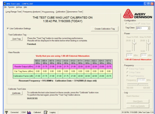
Figure 7: Test cube calibration procedure
