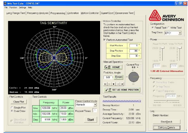
Figure 10: Angular response controls and plot
