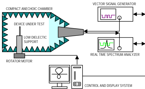
Figure 2: Primary response test system block diagram
