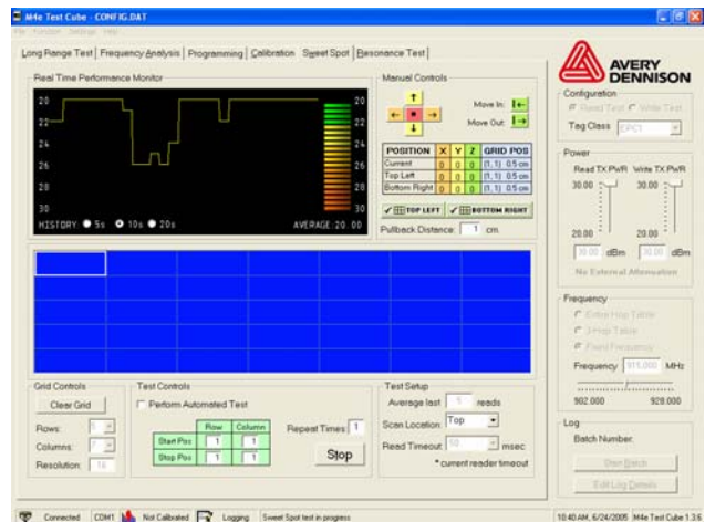
Figure 14: Display of sweep of sweet spot tester across a tray of bottled liquids
