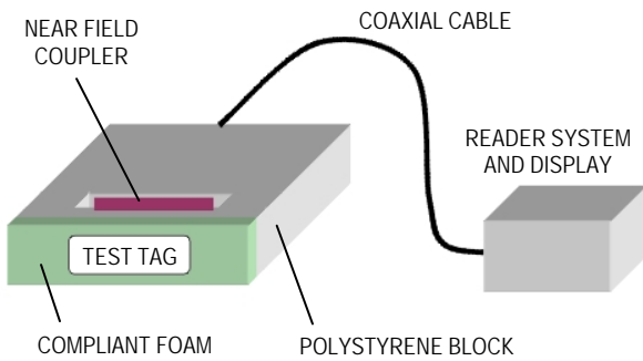
Figure 12: Sweet spot tester configuration
