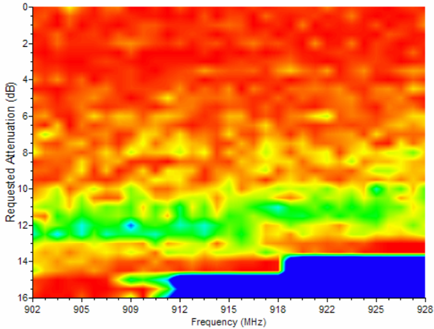
Figure 6: Inconsistent read probabilities of a reader at various powers and frequencies.
