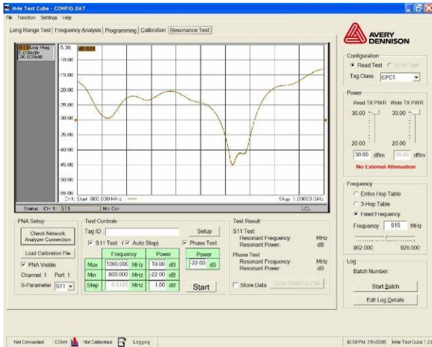
Figure 8: Measuring resonance frequency by running test cube control software on network analyzer
